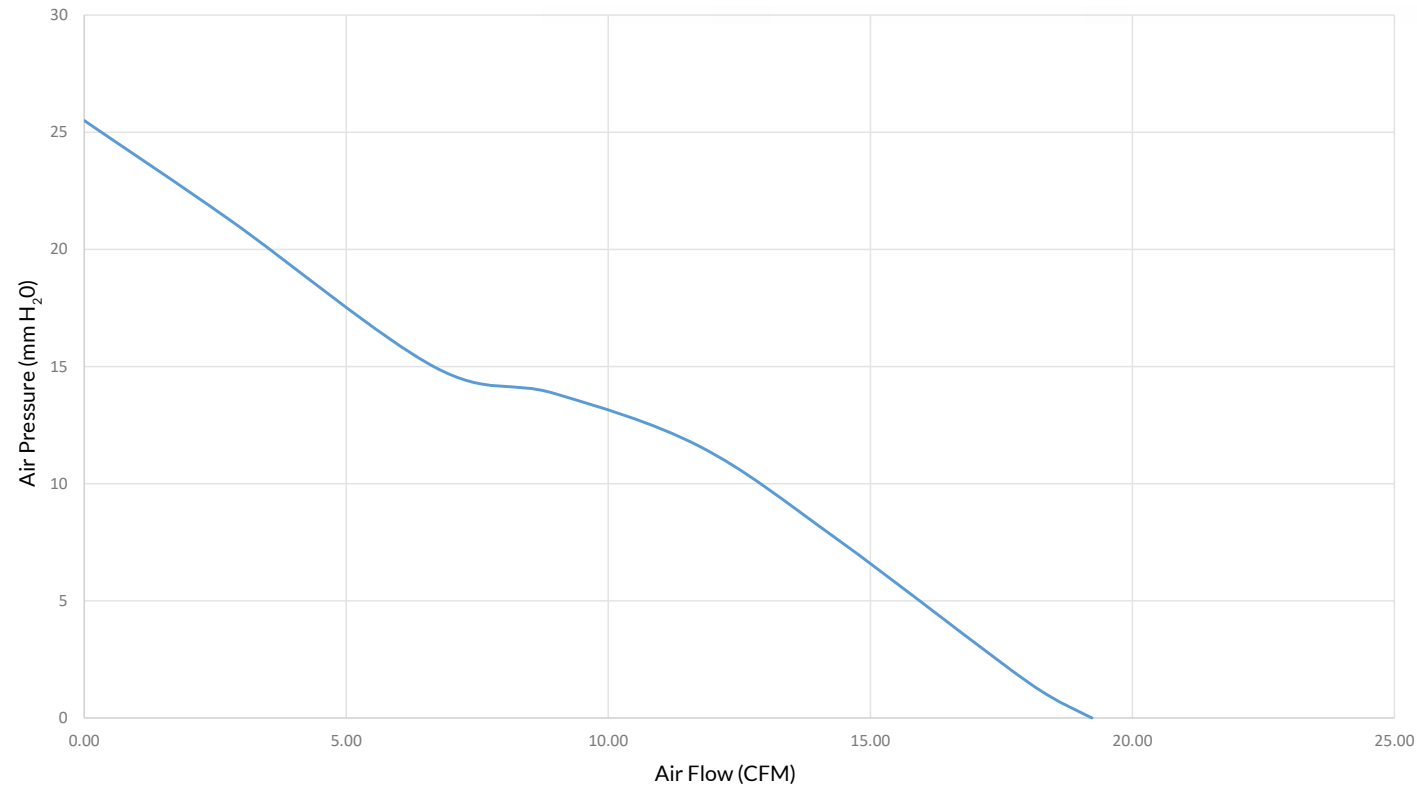
P/Q Curve
