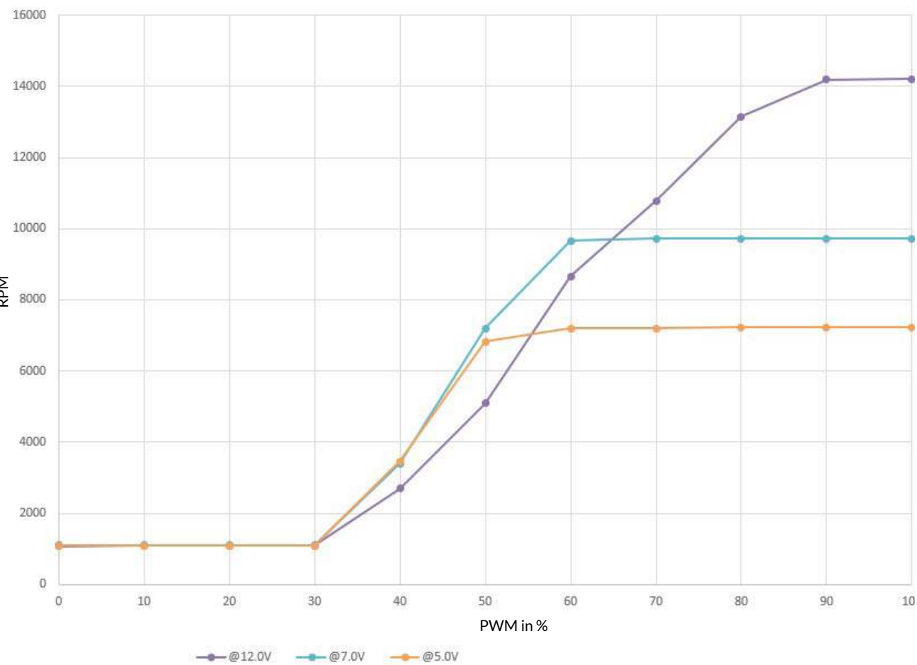
PWM to rpm Curve
